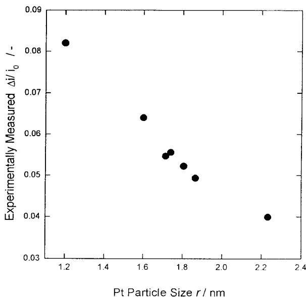
Fig. 3. Plot of the value of \Delta i/i_0 determined from the cathodic potentiostatic current transients obtained just after stepping the OCP down to 0.4 V vs RHE as a function of Pt particle size r .
